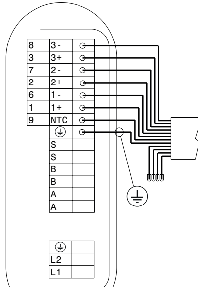
GWP30032 - DMX
